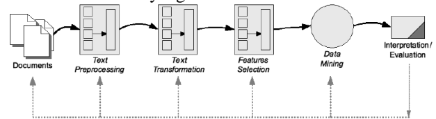
Gambar 2.1 Alur Proses Text Mining
