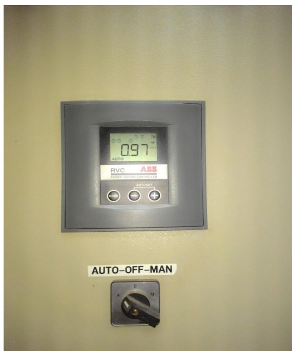
Gambar : Pengukuran Faktor Daya di Power Factor Regulator Saat Capasitor Bank
