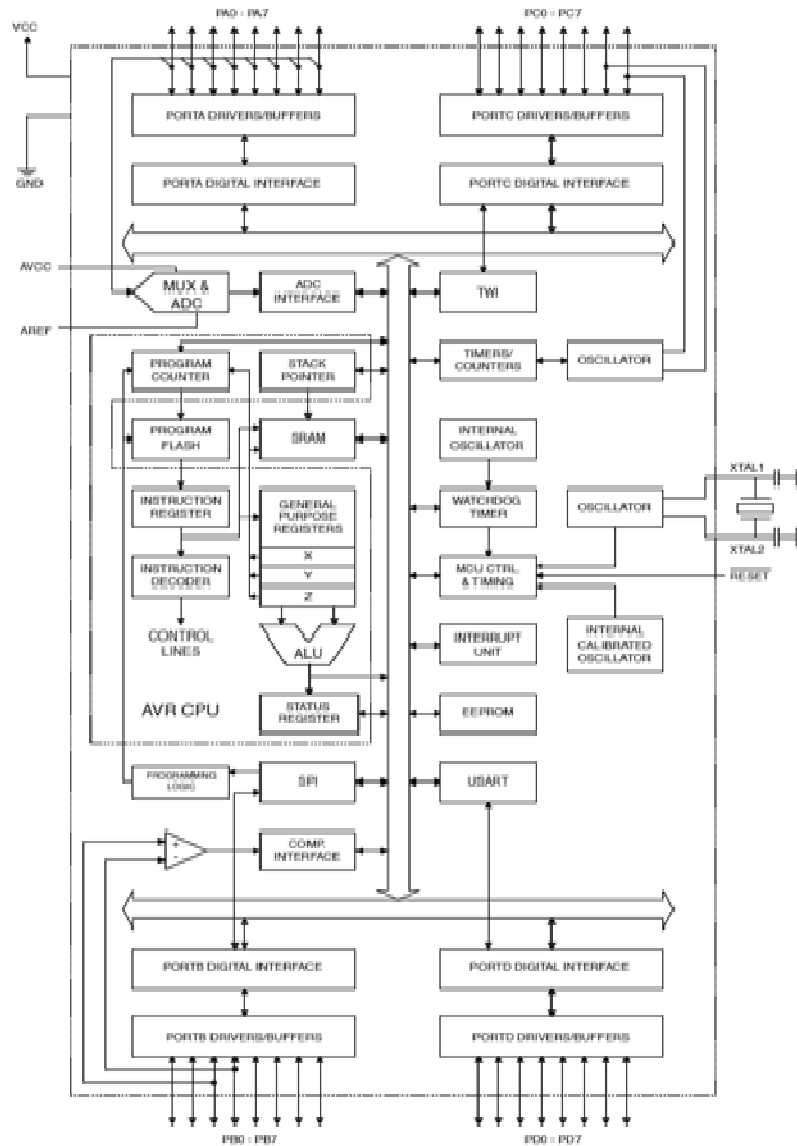
Figure 2. Block Diagram
