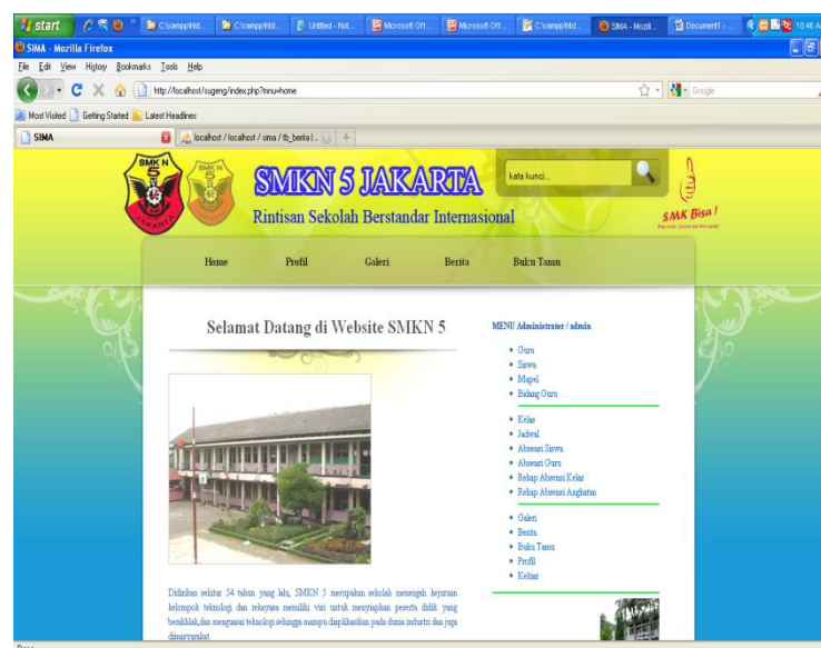
Gambar 4.3 Halaman admin
