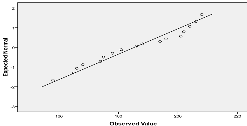
Normal Q-Q Plot of X1_X2_X3
